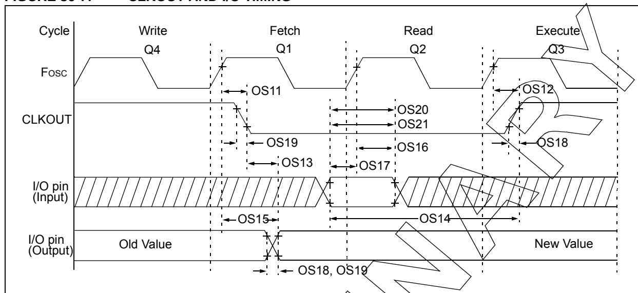
FIGURE 36-7: CLKOUT AND I/O TIMING
