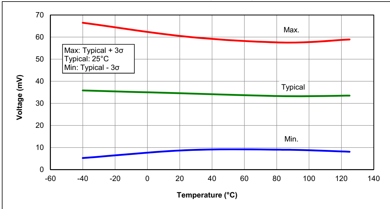
FIGURE 37-12: BROWN-OUT RESET HYSTERESIS, BORV = 1, PIC16F1777/8/9 ONLY
