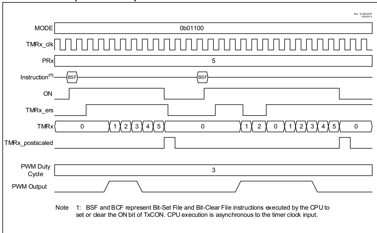
FIGURE 23-10: EDGE-TRIGGERED HARDWARE LIMIT ONE-SHOT MODE TIMING DIAGRAM (MODE = 01100)
